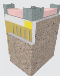
Outside Corner
