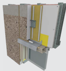
Window Box Head Flashing Integration
