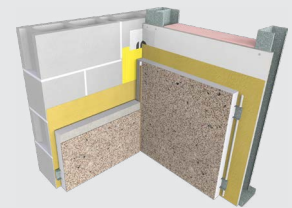
Inside Corner - Dissimilar Existing Wall Types (Masonry to Metal Frame)
