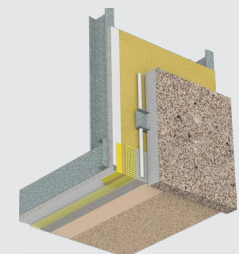
Soffit Termination
