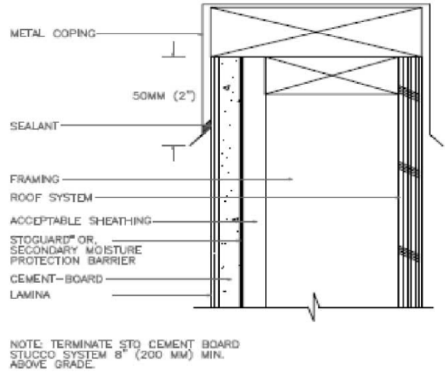
FIGURE 4—TYPICAL METAL COPING DETAILS
