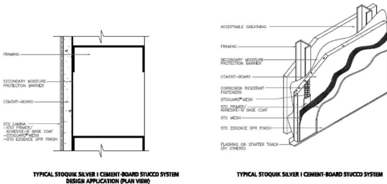
FIGURE 1—STOQUIK™ SILVER I CEMENT-BOARD STUCCO SYSTEM
