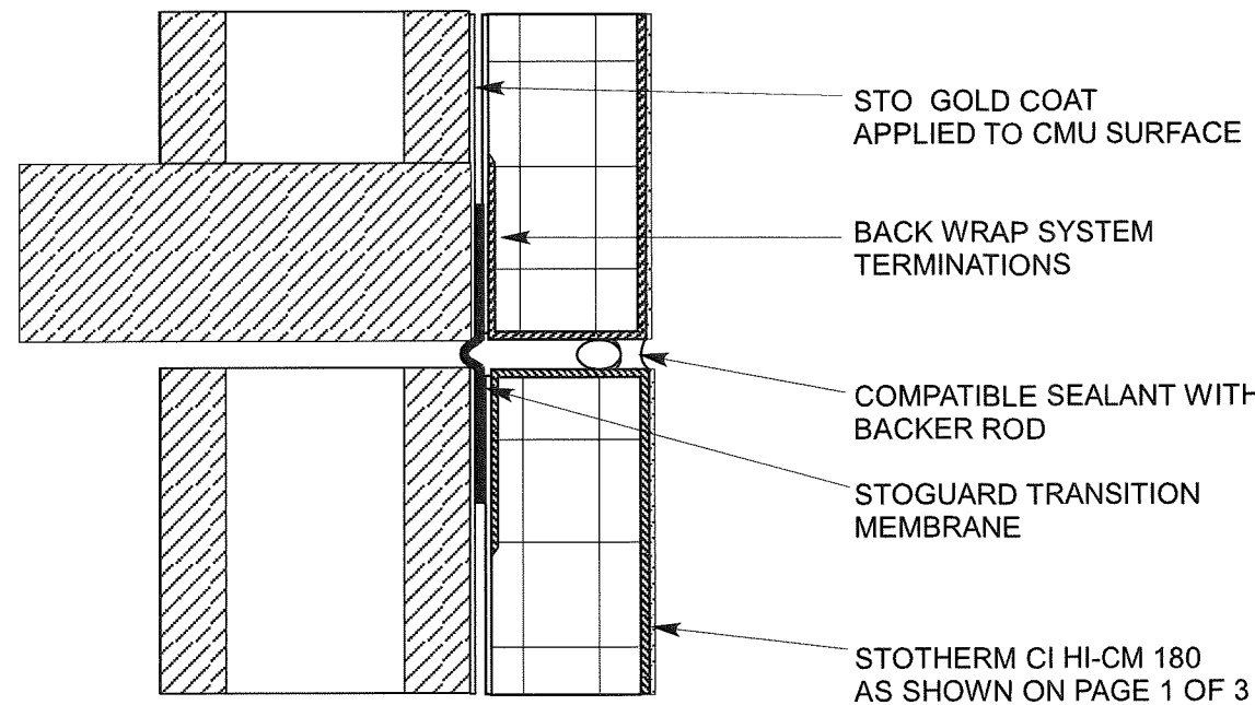
FLOOR LINE SEALANT JOINT
