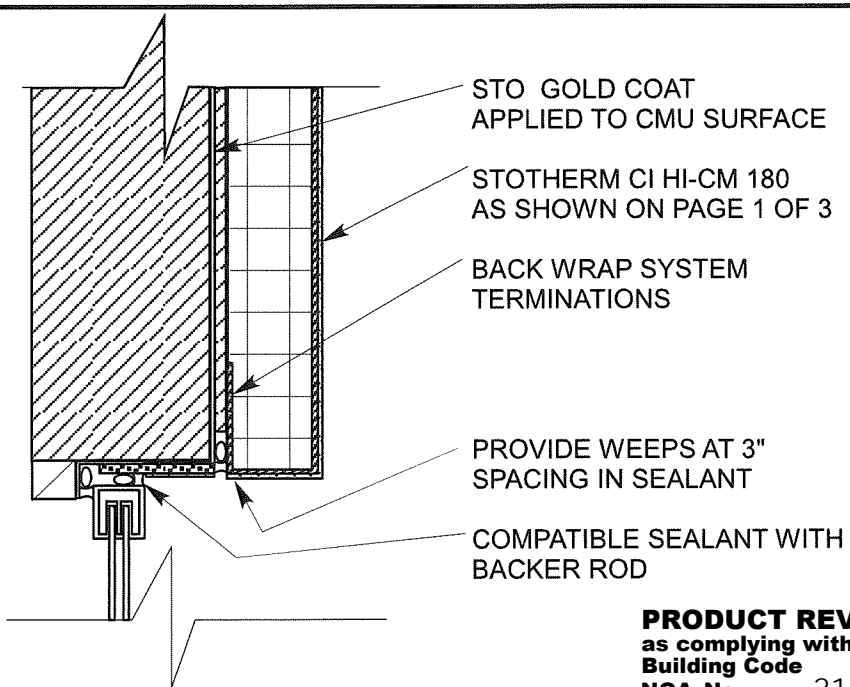
WINDOW HEAD
