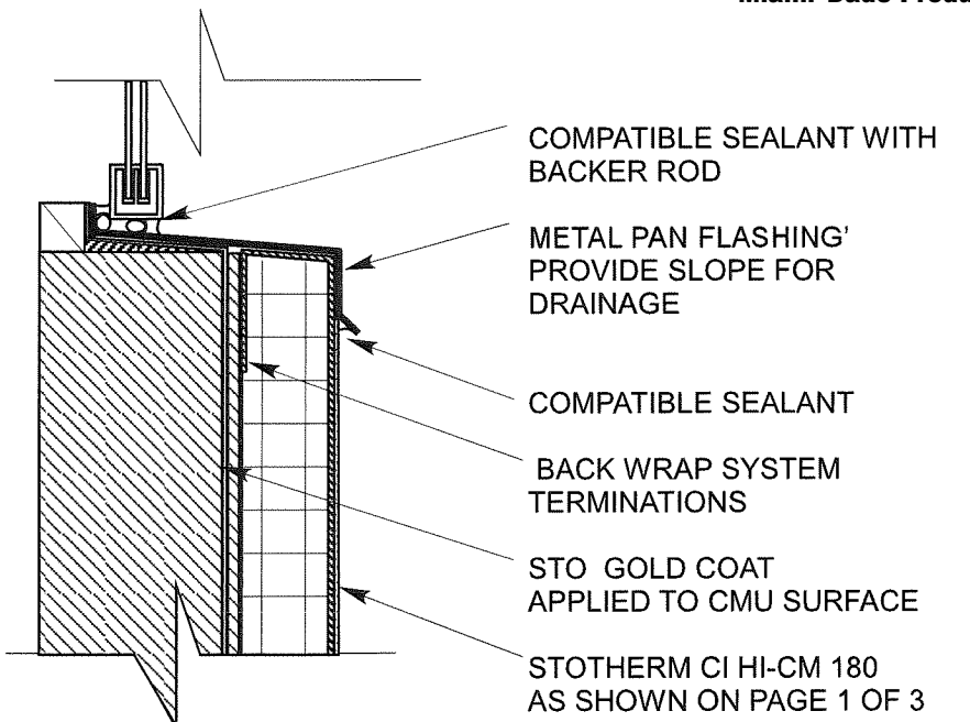
WINDOW SILL
